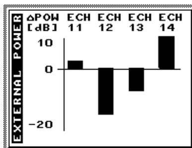
Fig. 2-173 Display of external power control mode
