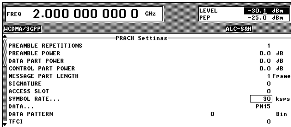
Fig. 2-120 DIGITAL STD – WCDMA/3GPP – MS CONFIGURATION: PRACH only Mode menu
