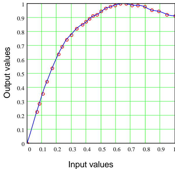
Fig. 2-241 AM/AM conversion
