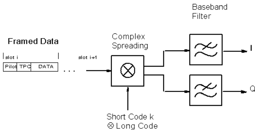
Fig. 2-88 Downlink DPCH signal generation for a code channel
