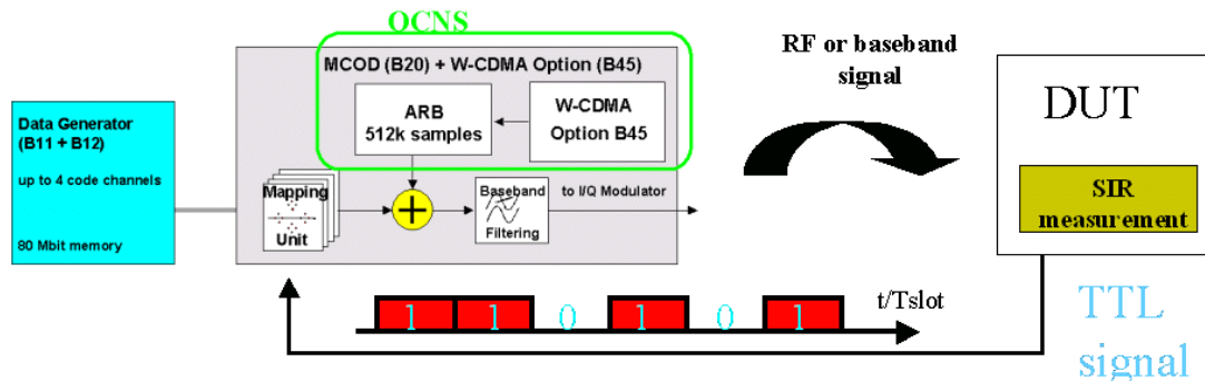
Fig. 2-170 Setup for testing Closed Loop Power Control
