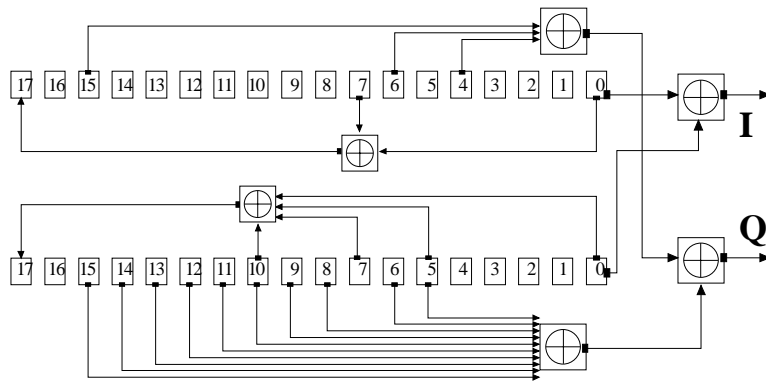
Fig. 2-98 Structure of the downlink scrambling code generator
