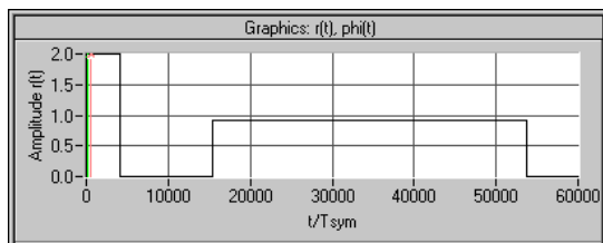
Fig. 2-145 Envelope of a PRACH
