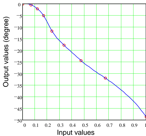
Fig. 2-242 AM/PM conversion
