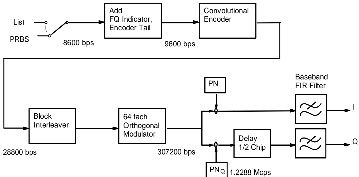
Fig. 2-78 Traffic channel 9600 in "Reverse Link Coded" mode
