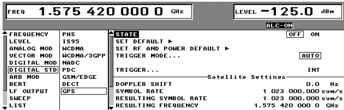
Fig. 2-212 DIGITAL STD - GPS menu
