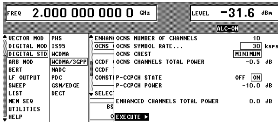
Fig. 2-174 DIGITAL STD - WCDMA/3GPP - OCNS CHANNELS menu
