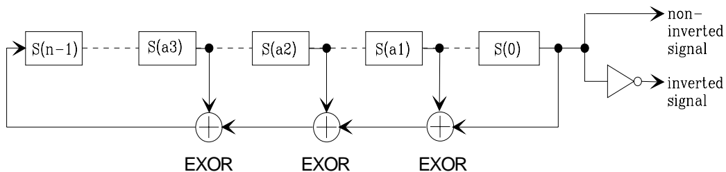
Fig. 2-236 PRBS polynomials
