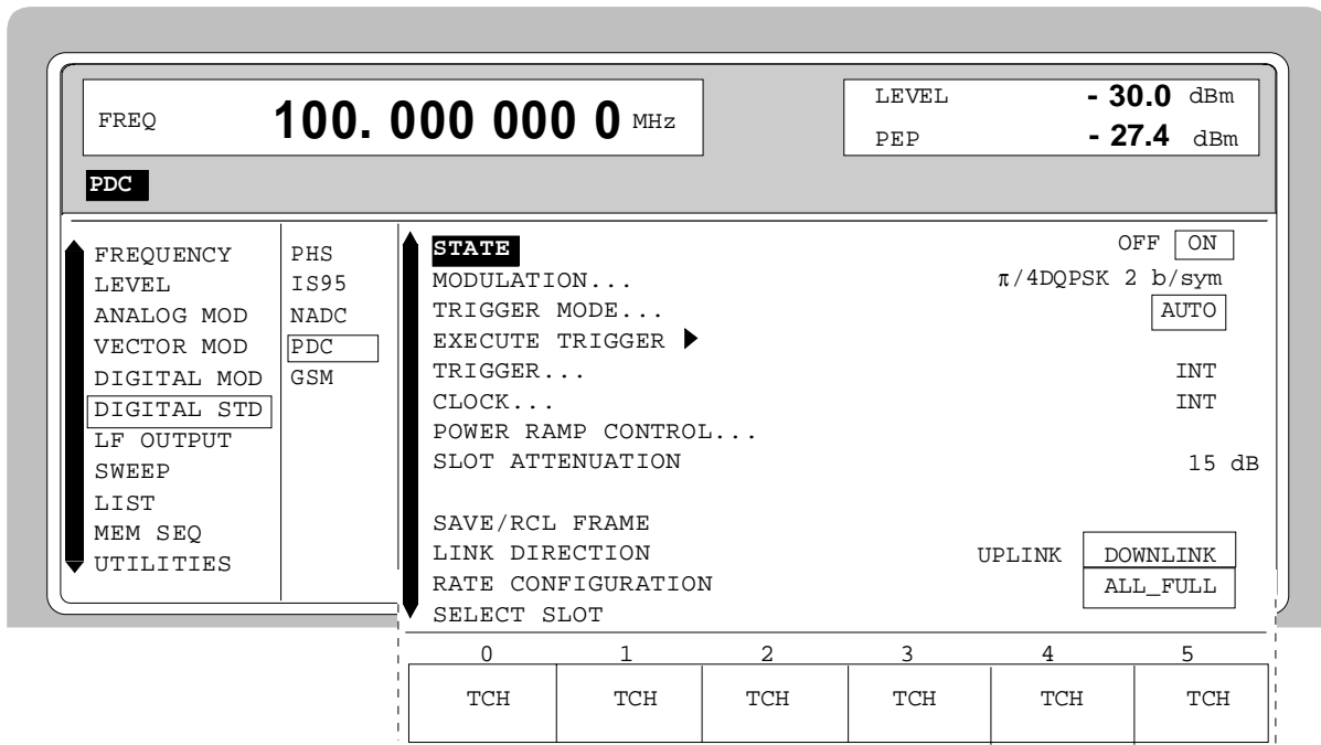
Fig. 2-185 Menu DIGITAL STD - PDC, SMIQ equipped with Modulation Coder SMIQB20 and Data Generator SMIQB11
