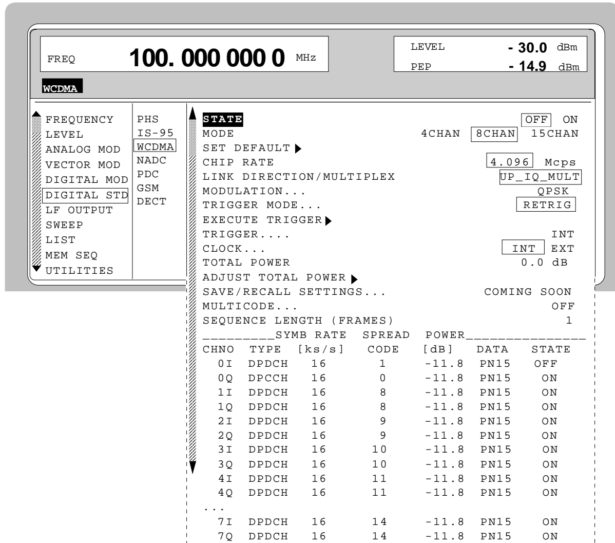
Fig. 2-96 Menu DIGITAL STD - WCDMA - MODE - 8CHAN, -LINK DIRECTION/MULTIPLEX - UP_IQ_MULT, equipped with options modulation coder SMIQB20, data generator SMIQB11 and SMIQB43
