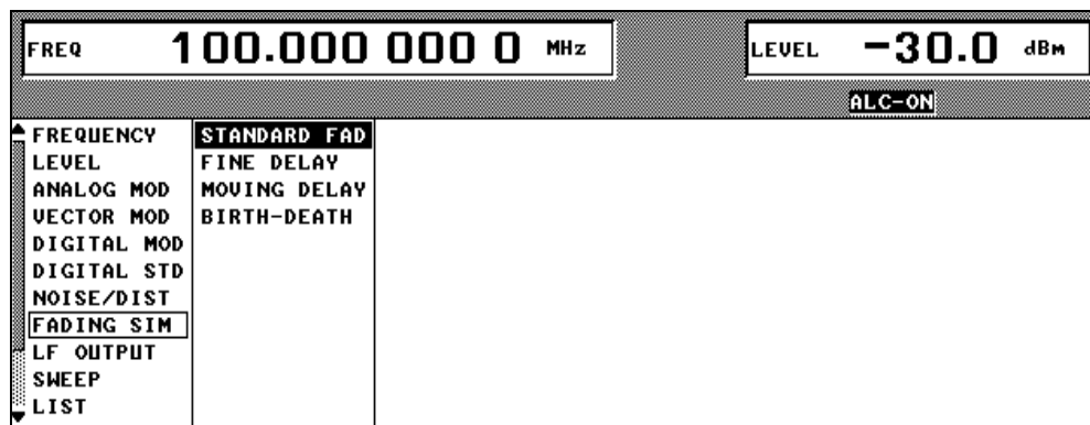
Fig. 2-38 Menu FADING SIM with submenus
