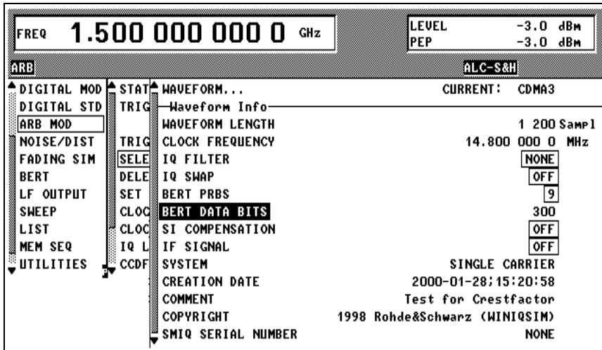
Fig. 2-221 ARB MOD - WAVEFORM INFO menu
