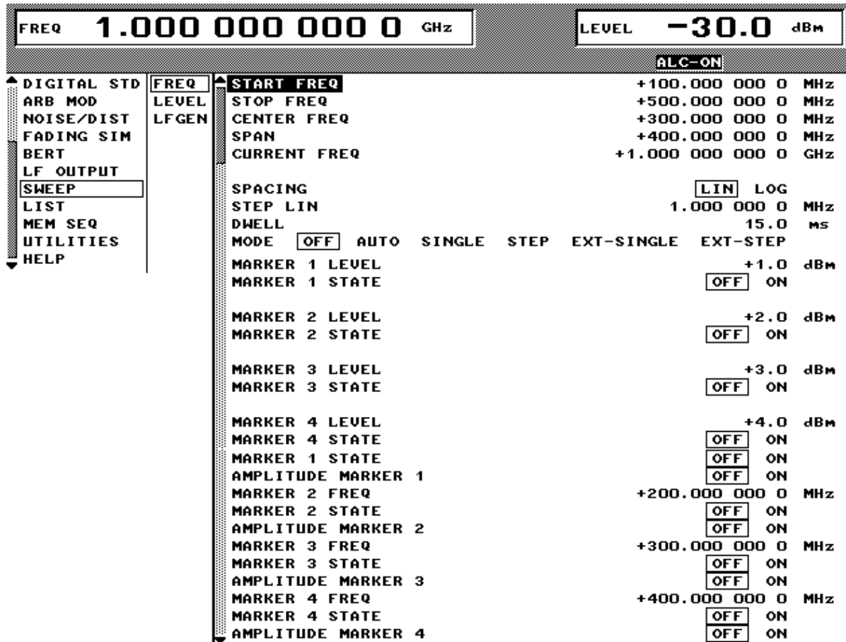
Fig. 2-246 Menu SWEEP - FREQ
